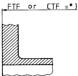
Figure 2. Flat face flange
