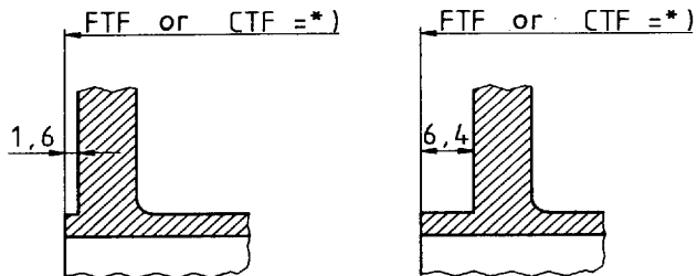
Figure 3. Raised face flange
