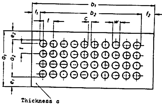
Figure 3. Rg round holes in straight rows
