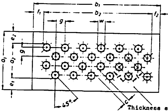
Figure 2. Rd round holes in diagonally staggered rows
