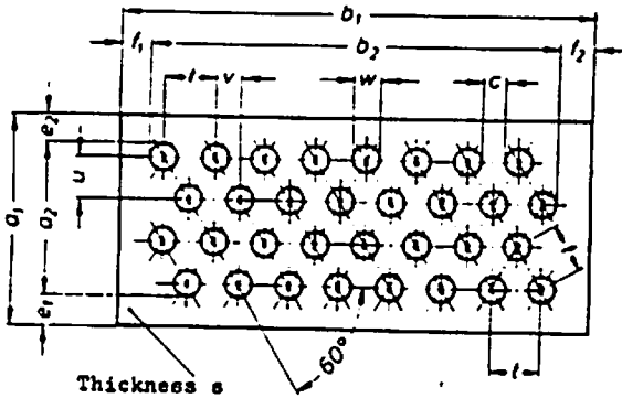
Figure 1. Rv round holes in staggered rows
