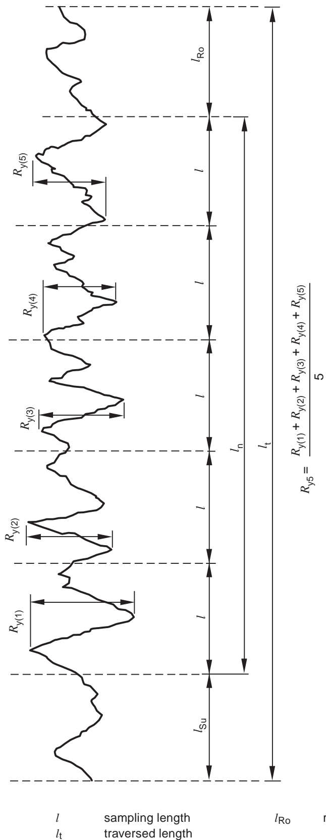
Figure 1 — Components of a stylus profile measurement on a blast-cleaned surface
